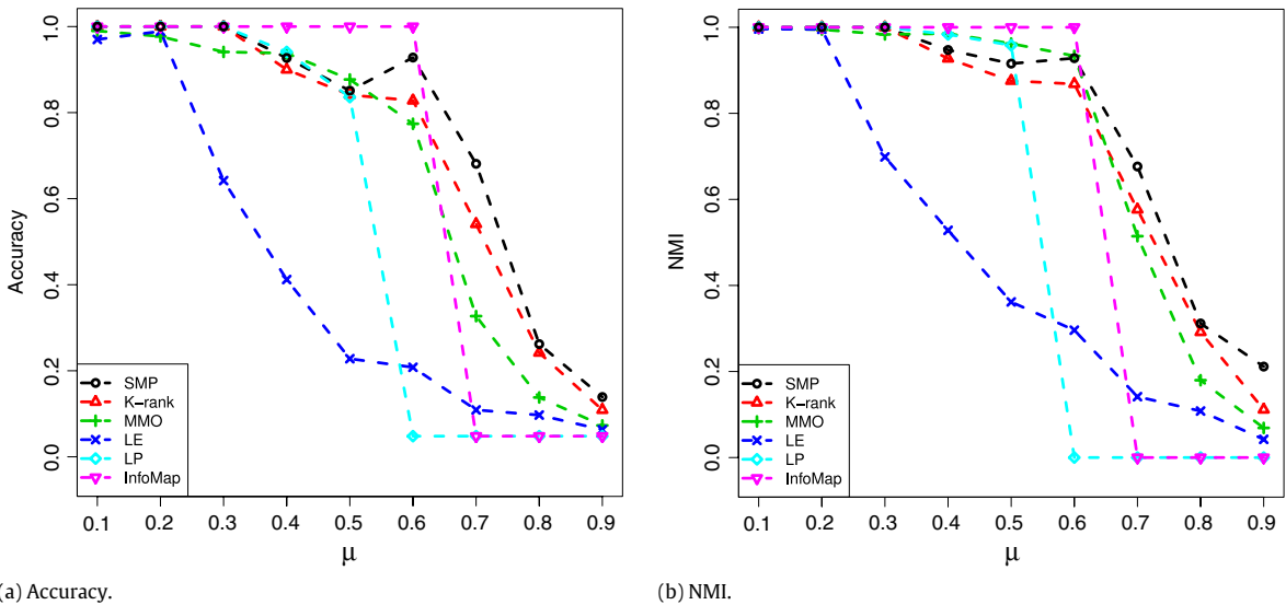
Fig. 4. Comparison of SMP and other algorithms in LFR networks. The number of nodes is N = 1000 . The average degree is \langle k \rangle = 20 , and the pair for the exponents is (\gamma, \beta) = (2, 1) .
