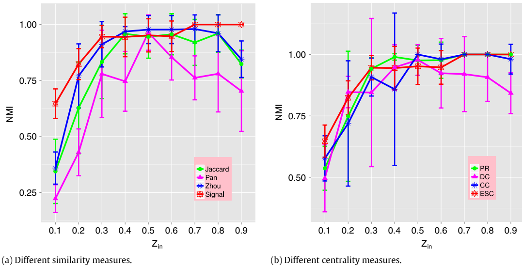
Fig. 2. Comparison of similarity and centrality measures in the application of SMP algorithm. Average NMI values (plus and minus one standard deviation) for 20 repeated experiments, as a function of the average degree.
