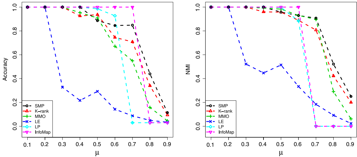
Fig. 5. Comparison of SMP and other algorithms in LFR networks. The number of nodes is N = 2000 . The average degree is |k| = 30 , and the pair for the exponents is (\gamma, \beta) = (2, 1) .
