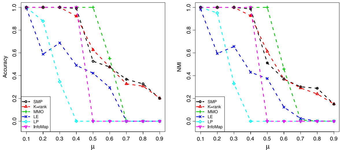
Fig. 6. Comparison of SMP and other algorithms in LFR networks. The number of nodes is N = 5000 . The average degree is |k| = 30 , and the pair for the exponents is (\gamma, \beta) = (2, 1) .
