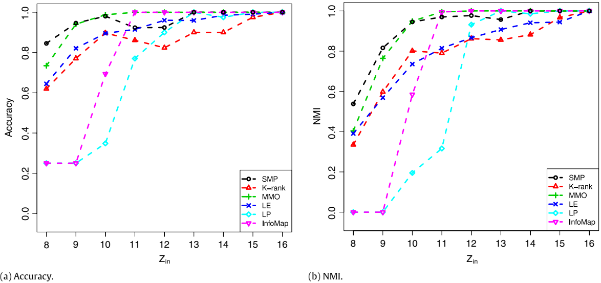
Fig. 3. Comparison of SMP and other algorithms in Girvan and Newman's networks.
