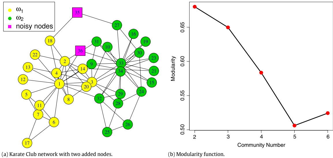
Fig. 8. The Karate Club network with added nodes and the modularity values varying with community numbers.
