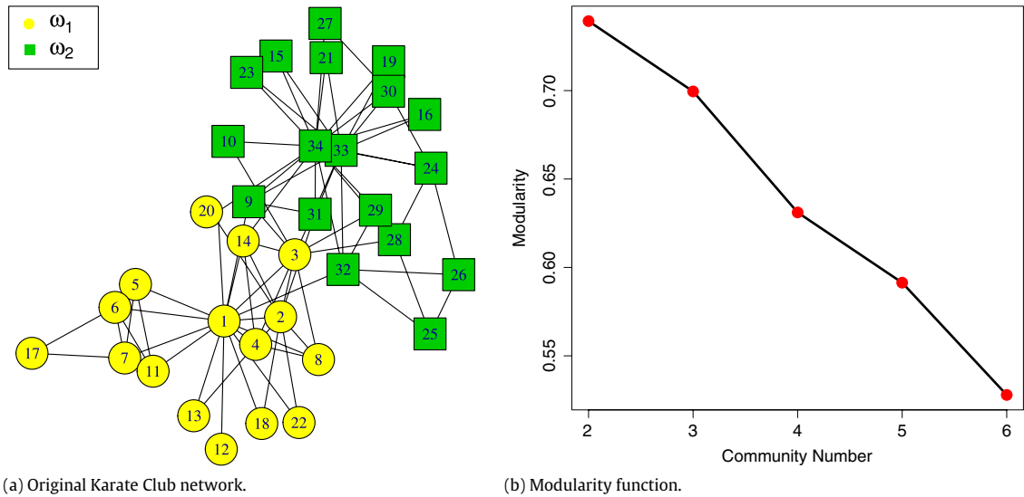
Fig. 7. The Karate Club network and the modularity values varying with community numbers.
