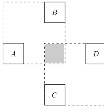
Figure 9.1: Non-distributivity.
